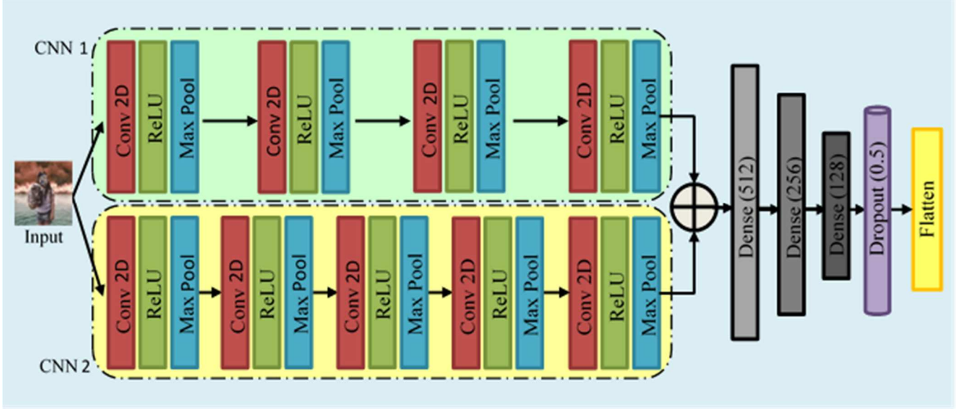
Fig 3. Proposed architecture of Multiscale Convolutional Neural Network
